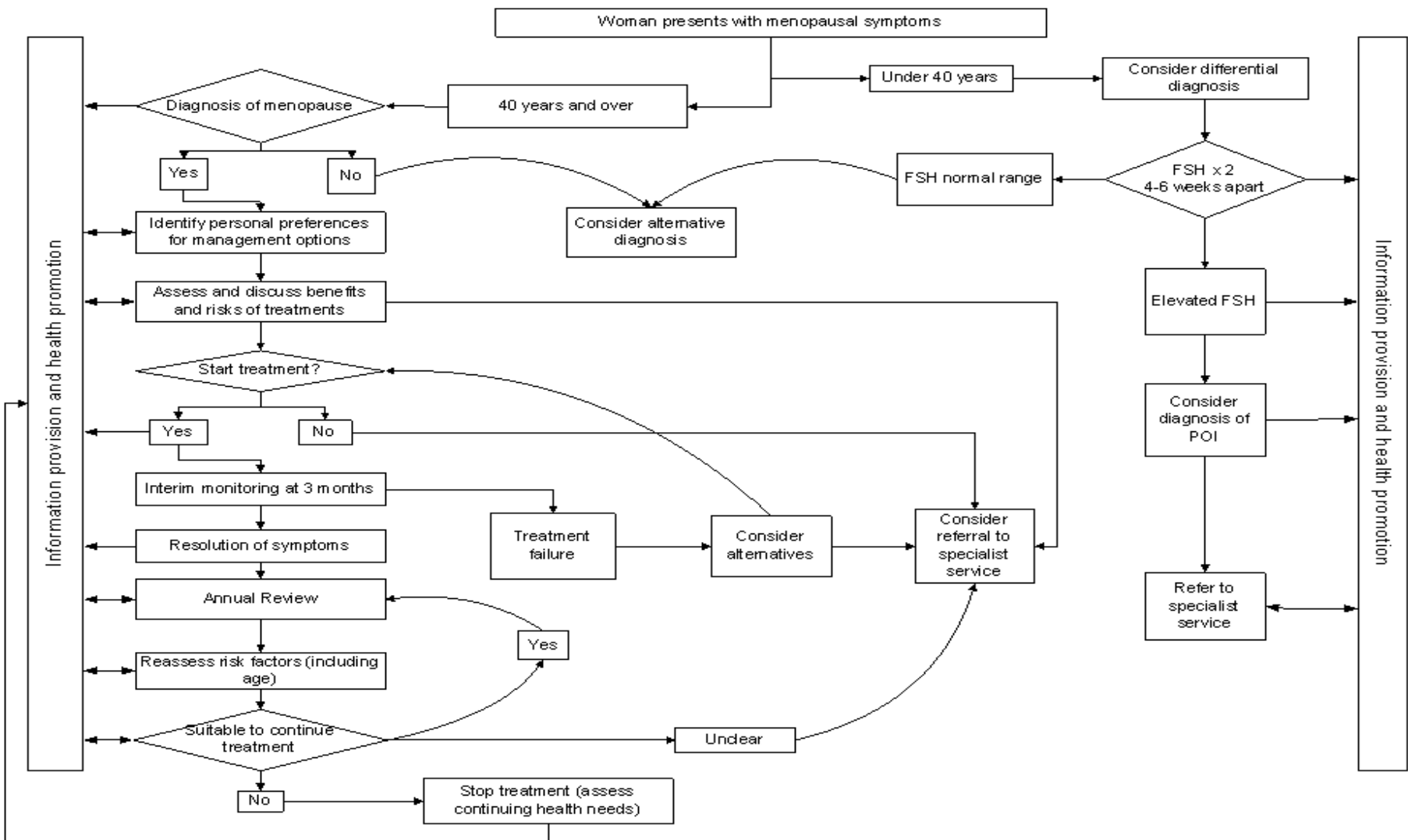
Figure 1: Care algorithm
